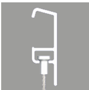
Coupling with T-sleeve 02, inserted laterally. See page 21
